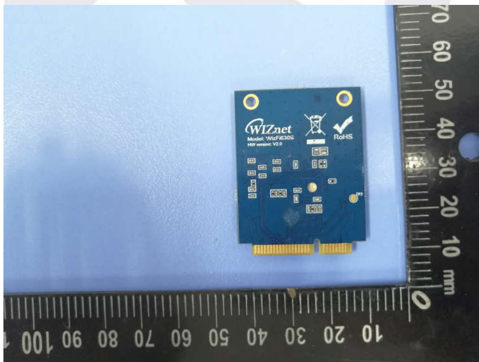
Model WizFi630S overview II
