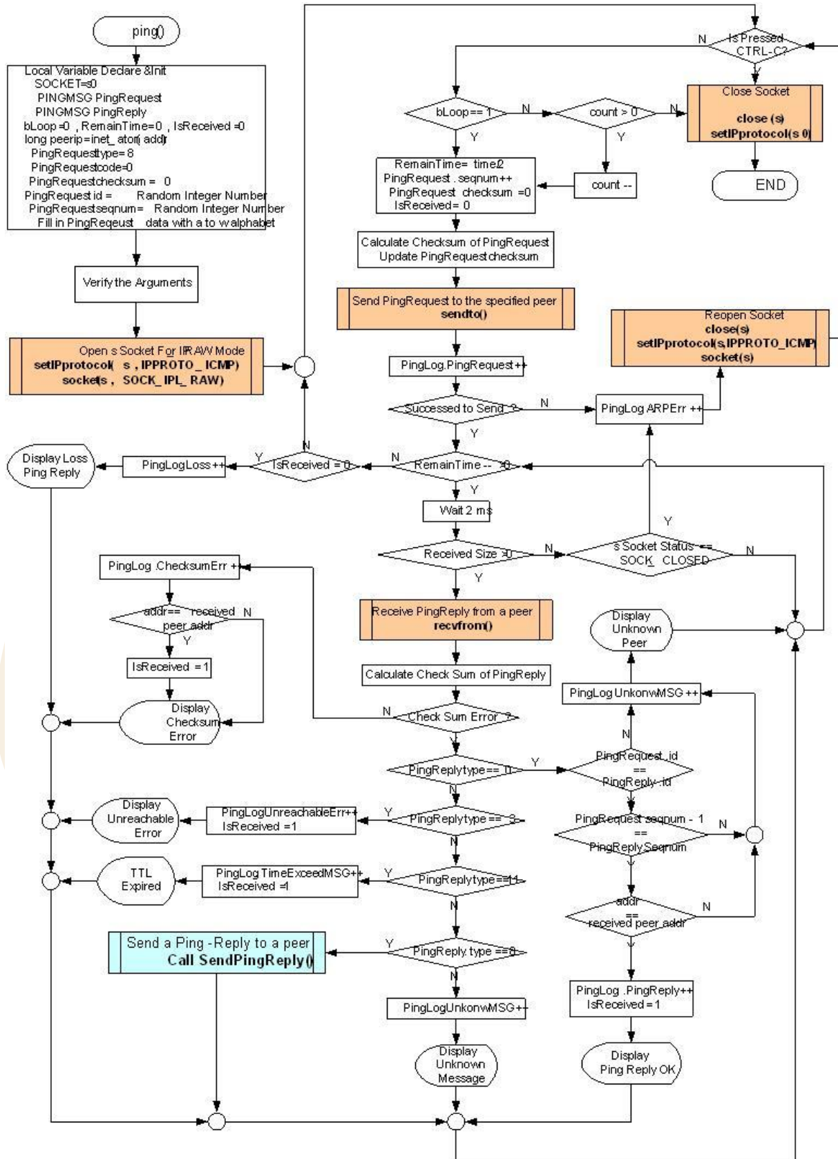
<Fig 3.11: ping(>
