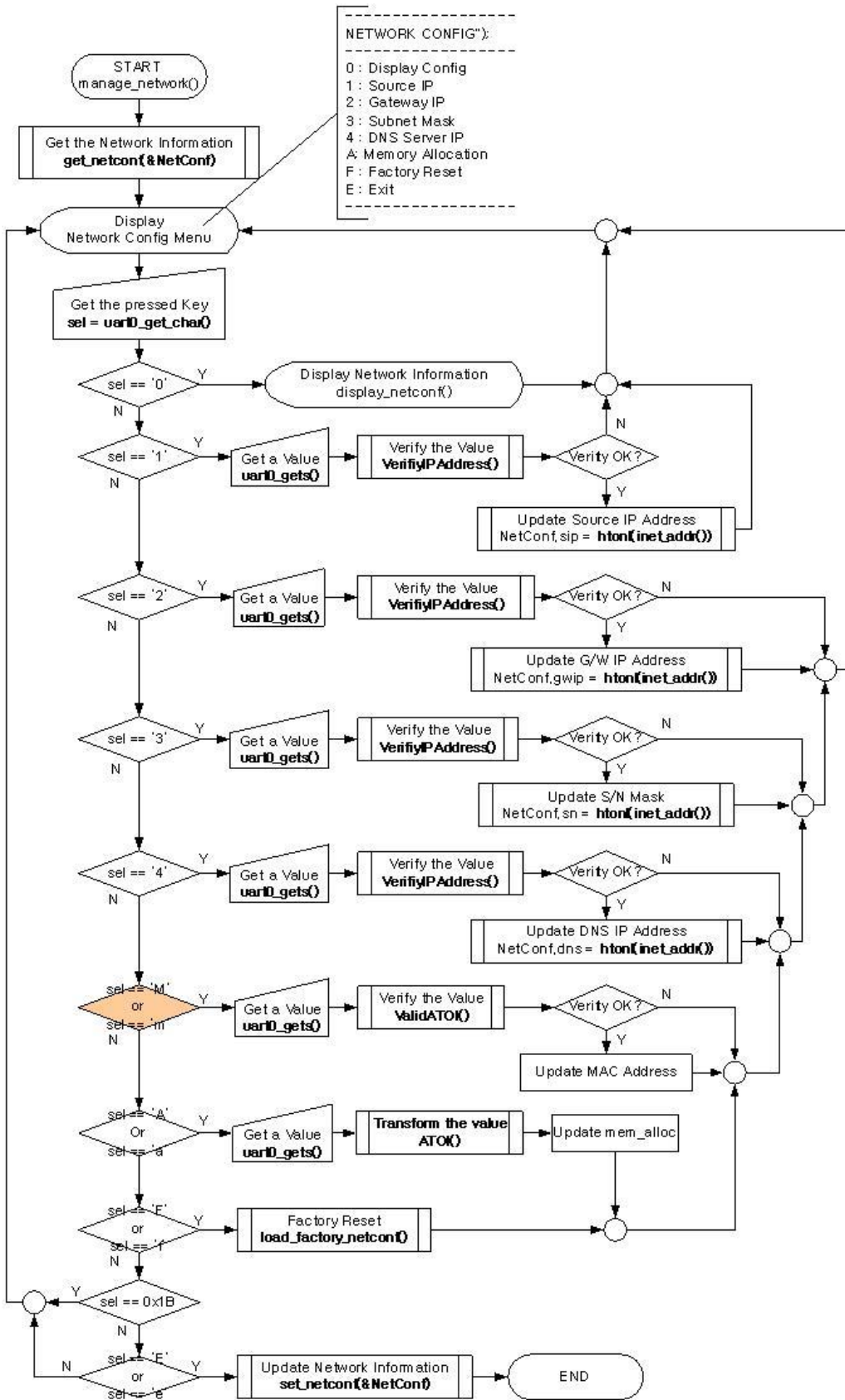
<Fig 3.6: manage_network()>
