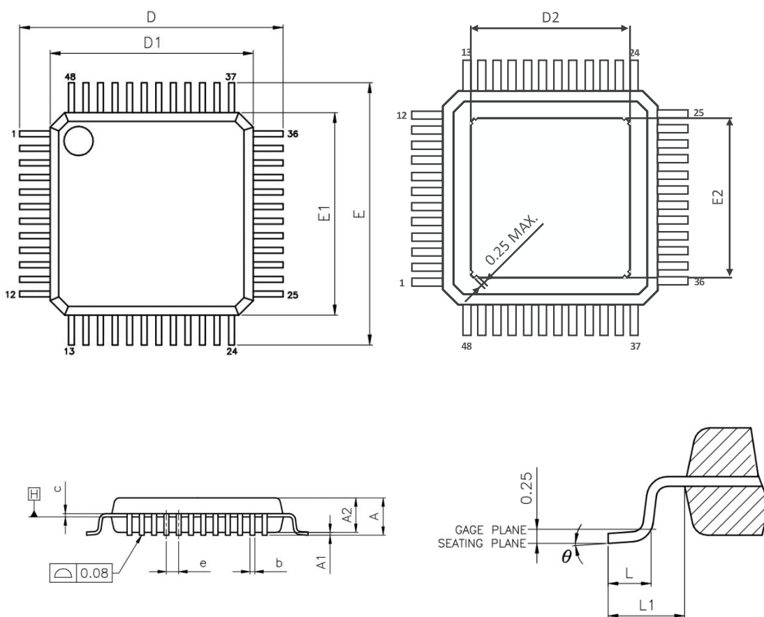
Figure 39 48LQFP (EPAD) Dimension
