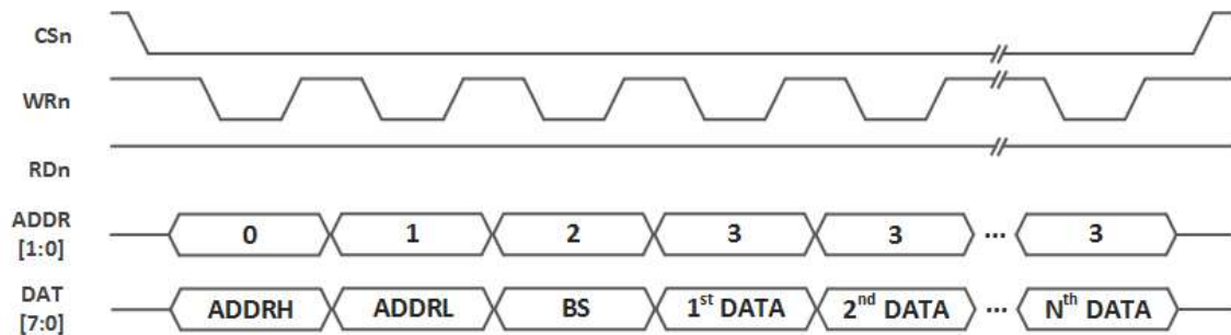
Figure 13 Parallel BUS N-Bytes Data Write Access
