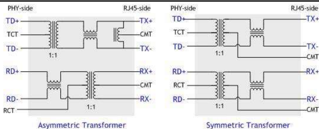
Figure 33 Transformer Type
