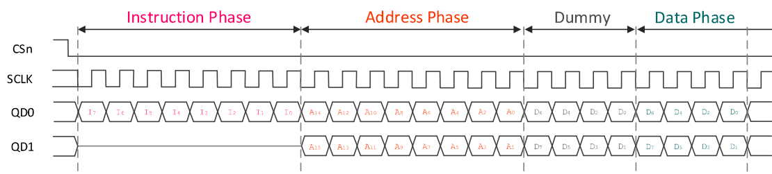
Figure 10 Dual SPI Frame Format
