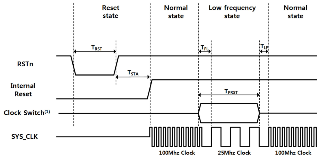
Figure 34 Reset Timing
